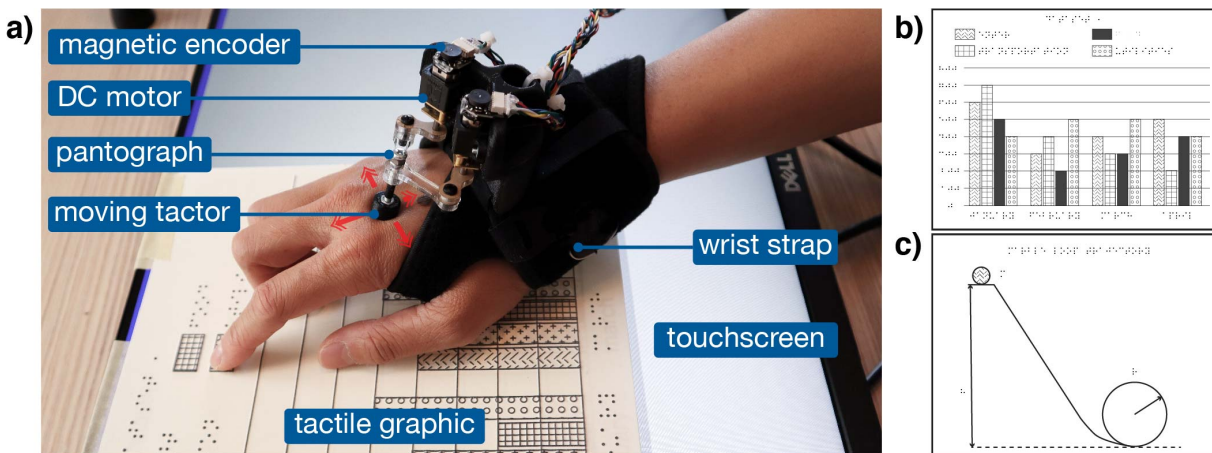
Figure 1: a) PantoGuide is a system that provides haptic and audio guidance cues to a user while exploring a tactile graphic. The device has a tactor in contact with the user that moves in a 2D plane (red arrows) to provide skin-stretch feedback. We demonstrate its use in two applications: b) providing point-to-point directional guidance cues when a user explores different elements of a tactile bar chart, and c) providing continuous guidance on the trajectory of a moving marble
