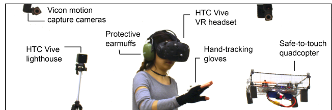
Figure 10: Experimental Setup.
