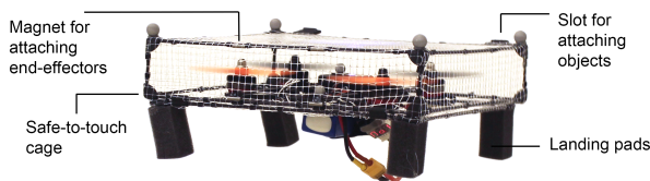
Figure 8: Safe-to-touch quadcopter with the protective cage.
